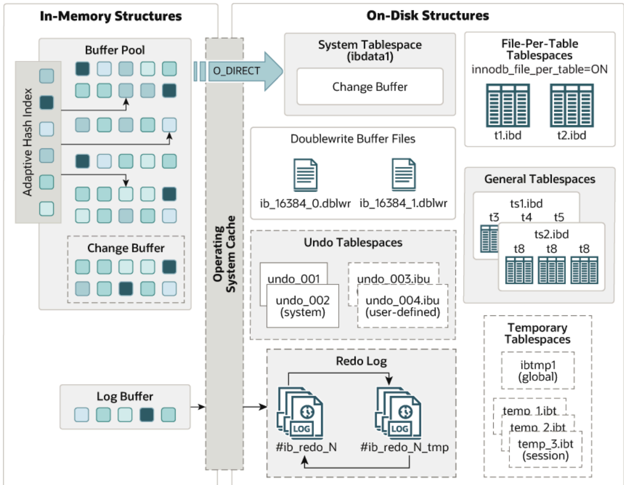
Figure 17.1 InnoDB Architecture
